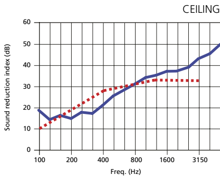
Rating according to ISO 717-1 Rw = 29 dB
